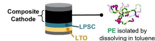
Fig. 5 (a) Fabrication of composite cathode and solid-state cell configuration, LTO|Li 6 PS 5 Cl|NMC-PE composite. (b) Specific discharge capacity vs. cycle number at T = 60 °C, 1 MPa stack pressure, 1 mA cm -2 . (c) Initial discharge capacity, and capacity retention after 200 cycles (labelled).
