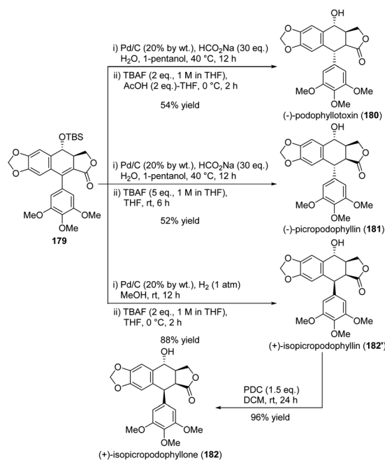
Scheme 45 Synthesis of aryltetrahydronaphthalen, (-)-podophyllotoxin, (-)-picropodophyllin, (+)-isopropodophyllin, (+)-isopropodophyllone from ADHN.
