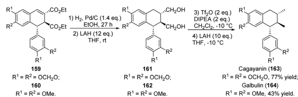
Scheme 40 Synthesis of aryltetrahydronaphthalene, cagayanin and galbulin via reduction reaction of ADHNs.
