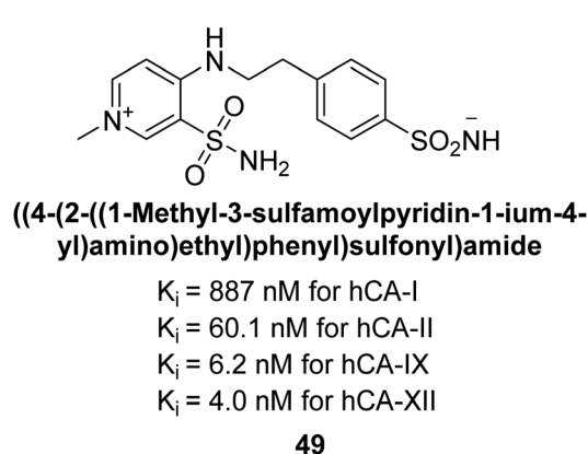
Fig. 19 Chemical structure of compounds 48 and 49 and their K_i values against hCA isoforms.
