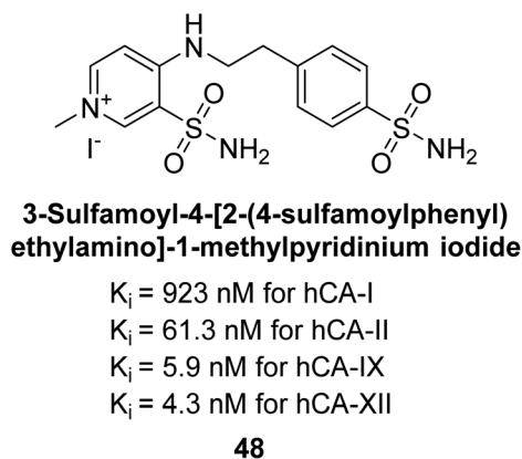
Fig. 19 Chemical structure of compounds 48 and 49 and their K_i values against hCA isoforms.
