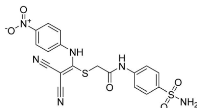
2-[2,2-Dicyano-1-(4-nitrophenylamino)vinylthio]-N-(4-sulfamoylphenyl)acetamide
