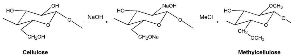
Fig. 8 The mechanism of methylcellulose synthesis. 162
