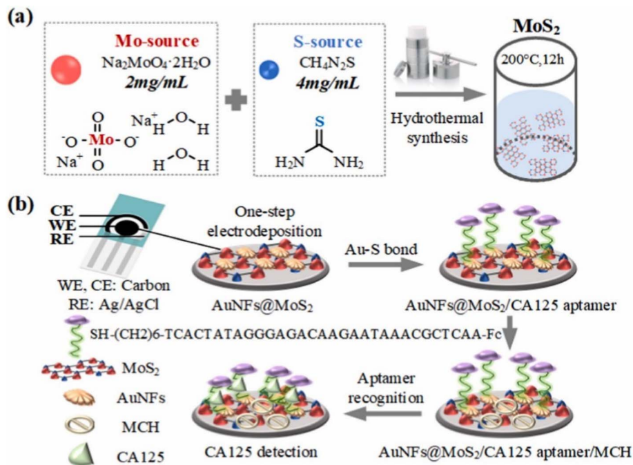
Fig. 7 Schematic diagrams of the sensing platform. (a) Synthesis of \text{MoS}_2 . (b) Modification of \text{AuNFs}@ \text{MoS}_2/\text{CA125} aptamer/MCH for CA125 detection. "This figure has been adapted from ref. 88 with permission from Elsevier, copyright 2023".
