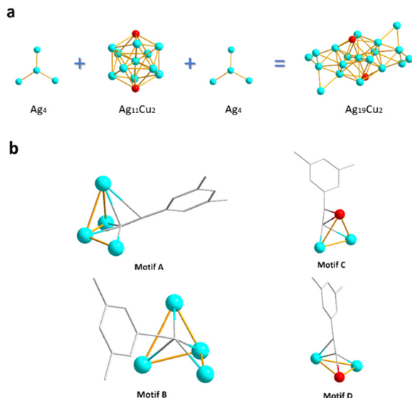
Fig. 2 (a) The structural anatomy of the \text{Ag}_{19}\text{Cu}_2 core. (b) Four different coordination modes between \text{Ag}/\text{Cu} and one alkyne molecule. Color legend: red, Cu; blue, Ag; green, Cl; purple, P; laurel green, F; white, H; gray, C.
