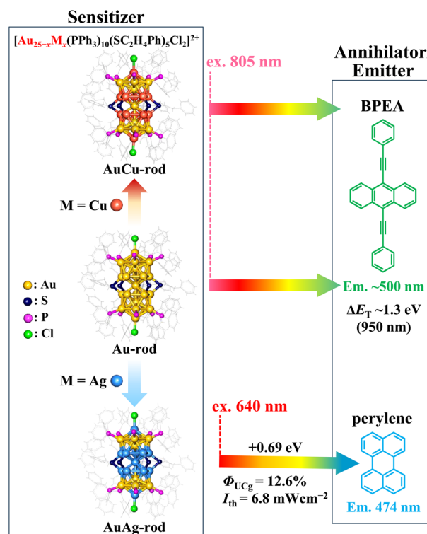
Scheme 2 [Au_{25}(PPh_3)_{10}(S-C_2H_4Ph)_5Cl_2]^{2+} ( Au-rod ) and its alloy nanoclusters, [Au_{25-x}Cu_x(PPh_3)_{10}(S-C_2H_4Ph)_5Cl_2]^{2+} ( AuCu-rod ) and [Au_{25-x}Ag_x(PPh_3)_{10}(S-C_2H_4Ph)_5Cl_2]^{2+} ( AuAg-rod ), were paired with the annihilator/emitter agents BPEA (for NIR-to-visible UC) and perylene (for red-to-blue UC), respectively. Chemical structures of these nanoclusters taken from ref. 30 and 31. The UC performance of AuAg-rod , taken from ref. 22, was also presented.
