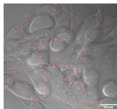
Fig. 6 Representative confocal images of the four types of cells after incubation with Rh-PE labeled liposomes of RGDK- and CGKRRK-lipopeptides. Cells were incubated (for 4 h) with Rh-PE labeled liposomes of RGDK- and CGKRRK-lipopeptides. (A) B16F10 cells; (B) HEK-293 cells; (C) RAW 264.7 cells; and (D) MDA-MB-231 cells. Representative red fluorescence images are shown (63x magnification). Scale: 20 μm. The details of the cellular uptake experiments are as described in the text.
