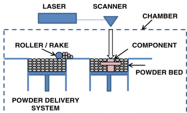
Fig. 4 Schematic of powder bed fusion. 60
