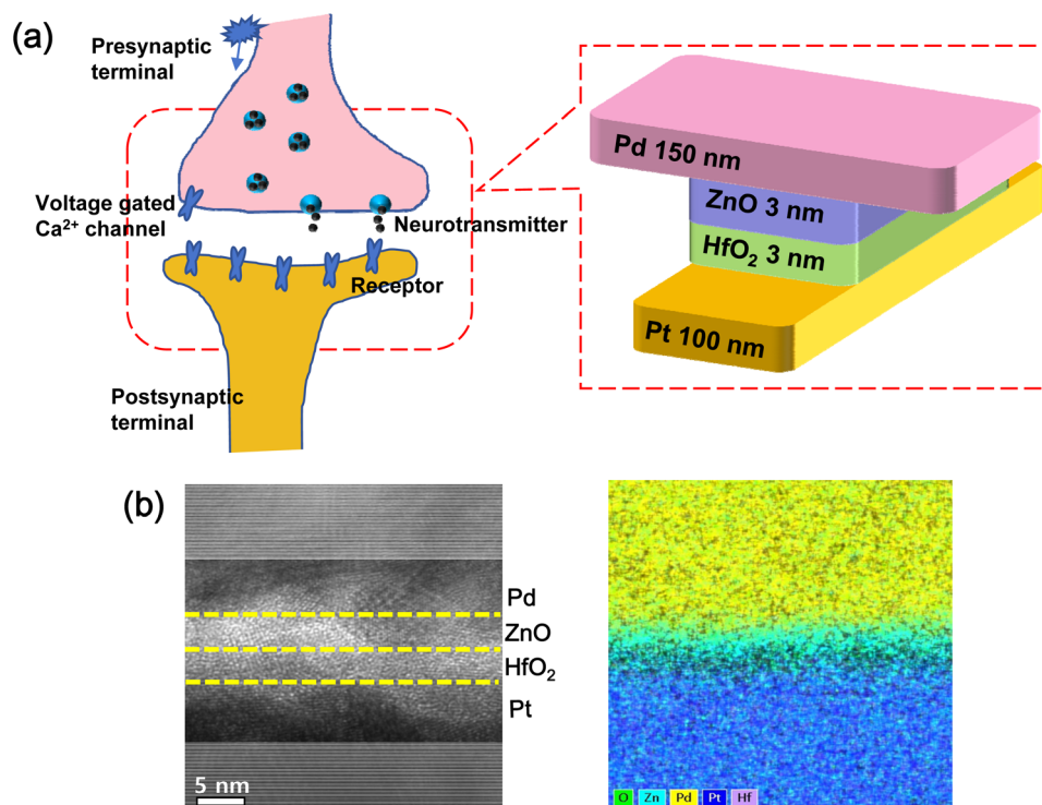
Fig. 1 (a) Schematic illustration of neurotransmission processes in a biological synapse and a 3-dimensional (3D) crossbar structure with a bilayer \text{HfO}_2 /ZnO synaptic device (artificial synapse), where the top Pd metal electrode mimics pre-synaptic neurons, and the bottom Pt metal electrode emulates post-synaptic neurons, (b) cross-sectional high-resolution transmission electron microscopy (HRTEM) and energy dispersive X-ray spectroscopy (EDS) images of bilayer \text{HfO}_2 /ZnO synaptic devices.
