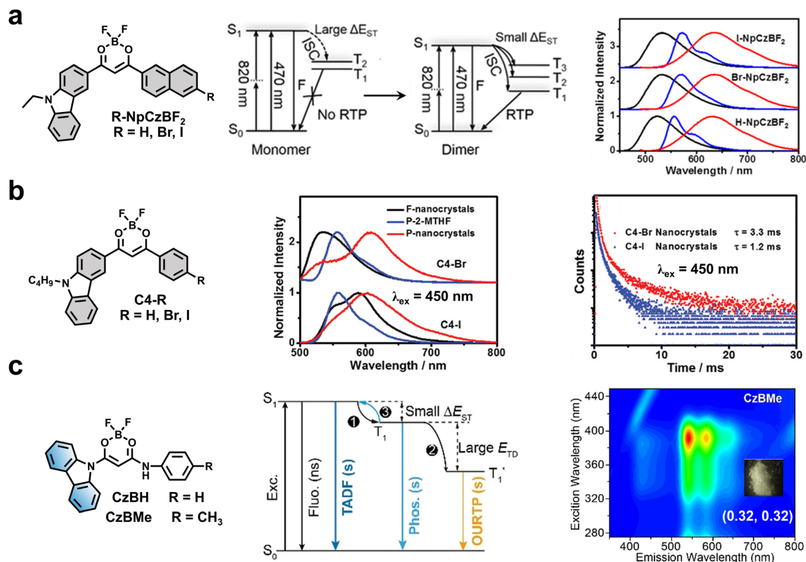
Fig. 6 (a) Visible- and NIR-light-excited RTP that combined with a difluoroboron \beta -diketonate unit (A) and a carbazoyl group (D). Reproduced with permission from ref. 28. Copyright 2019, American Chemical Society. (b) The D–A fluorogens for assembling visible-light-excited RTP nanocrystals, \lambda_{\text{ex}} = 450 nm. Reproduced with permission from ref. 51. Copyright 2020, Wiley-VCH. (c) The single-component D–A fluorogens enable white afterglow emission based on tri-mode emission. Reproduced with permission from ref. 52. Copyright 2021, Wiley-VCH.
