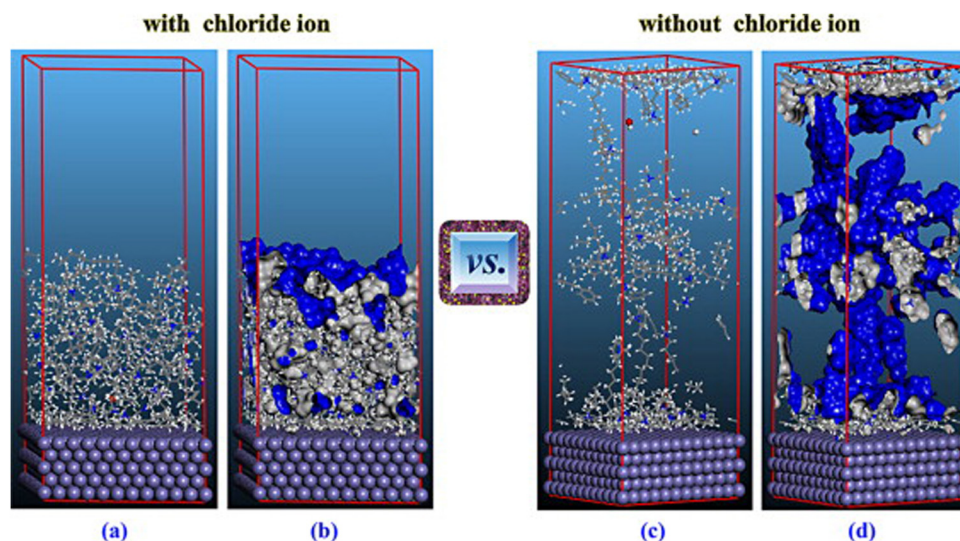
Fig. 22 (a) and (c) Equilibrium configuration and (b) and (d) free volume distribution of the inhibitor film of BKC cations with and without chloride ions.[Reprinted with permission from ref. 95, ©2015 Elsevier.]
