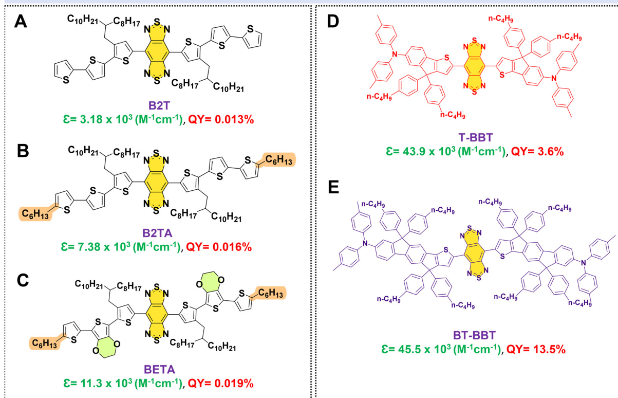
Fig. 11 D–A–D based fluorophores (A–E) with planar and twisted molecular architectures for high QY and high \epsilon .
