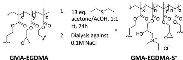
Scheme 1 The synthesis of sulfonium-functionalized GMA-EGDMA-S + was followed by dialysis against 0.1 M NaCl to exchange the acetate counter ion for a chlorine counter ion.
