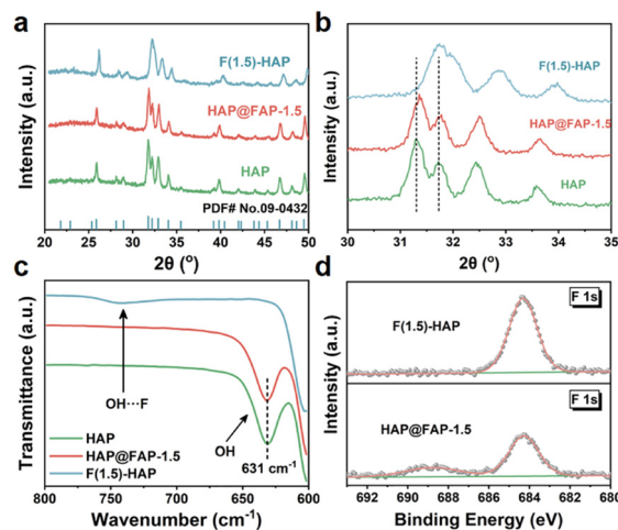
Fig. 3 (a) The XRD patterns of HAP, HAP@FAP-1.5, and F(1.5)-HAP; (b) enlarged view between 30-35^\circ ; (c) FTIR scans of HAP, HAP@FAP-1.5, and F(1.5)-HAP; and (d) F 1s high-resolution XPS spectra of HAP@FAP-1.5 and F(1.5)-HAP.
