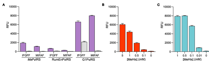
Fig. 3 Production of MeHis-containing GFP using engineered PylRS homologs. (A) Bar chart showing production of GFP containing MeHis at position 150, using either Ma PylRS MIFAF/IFGFF /Pyl t tRNA CUA , RumEnPylRS MIFAF/IFGFF /Pyl t tRNA CUA or G1PylRS MIFAF/IFGFF /Pyl t tRNA CUA pairs. Cultures grown in the presence of 0.5 mM MeHis (purple bars) or with no MeHis supplemented (grey bars). Error bars represent the standard deviation of measurements made in triplicate. (B) Bar chart showing GFP production in cultures containing varying MeHis concentrations (0–5 mM) using Ma PylRS IFGFF /Pyl t tRNA CUA . Error bars represent the standard deviation of measurements made in triplicate. (C) Bar chart showing GFP production in cultures containing varying MeHis concentrations (0–1 mM) using G1PylRS MIFAF /Pyl t tRNA CUA . Error bars represent the standard deviation of measurements made in triplicate.
