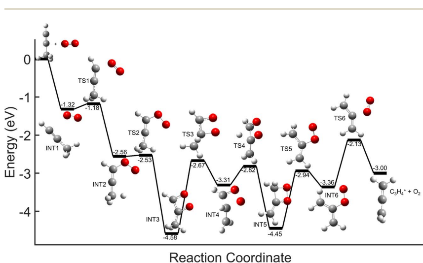
Fig. 8 Global potential energy surface of complex formation leading to \text{C}_3\text{H}_4^+ production for \text{O}_2^+ with propyne ( \text{H}_3\text{C}_3\text{H} ) calculated at the \omega\text{b97x/aug-cc-pvtz} level. All energies are displayed relative to reactant energy. Note that states INT1–INT4 are identical to those shown in Fig. 7. These surfaces have been separated for clarity.
