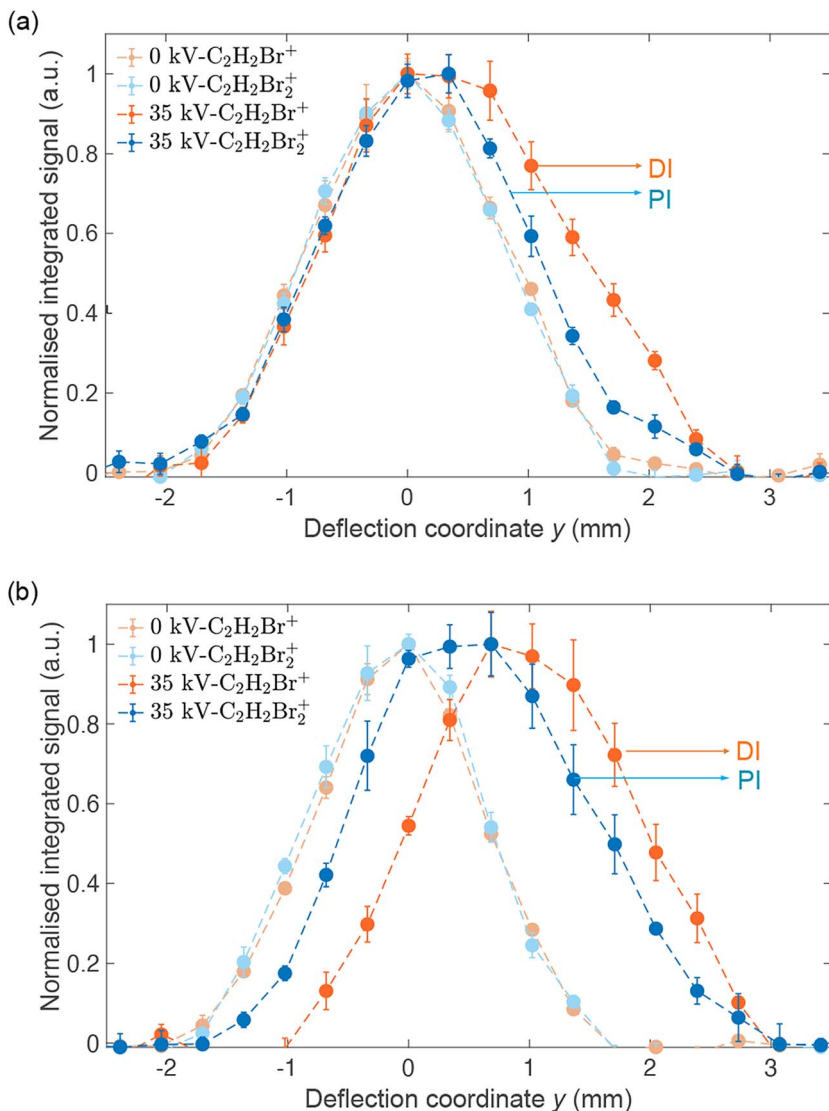
Fig. 4 Normalised reaction-deflection profiles of the CI of Ne* with (a) a \approx 1:1 mixture of cis-/trans -DBE and (b) pure cis -DBE at 0 kV (light symbols) and 35 kV (dark symbols) deflector voltage. Error bars denote the standard error of three individual measurements consisting of 5000 experimental cycles each. The profile of the DI product \text{C}_2\text{H}_2\text{Br}^+ is shifted with respect to the PI product \text{C}_2\text{H}_2\text{Br}_2^+ suggesting different dynamics for the two reaction channels. See text for details.
