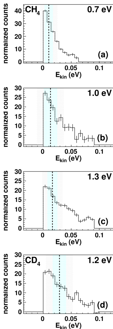
Fig. 3 Kinetic energy E_{kin} distributions for \text{TaCH}_2^+ (a–c) and \text{TaCD}_2^+ (d). The energy resolution is calculated using Gaussian error propagation from the energy and angular spread of the reactant beams. 54 The \pm 1\sigma -error interval is given by the light blue area and the \pm 2\sigma -error interval by the grey one. The distributions extend beyond the kinematic cut-offs given by energy and momentum conservation with respect to the relative collision energy E_{rel} and the reaction exothermicity E_{exo} . In other words, this means that an unavailable amount of energy is converted into kinetic energy. 71 Possible explanations are missing contributions to the energy balance, for example, electronically excited states of \text{Ta}^+ contributing or the internal energy of \text{CH}_4 . The relative contributions of events scattered within the kinematic cut-off and the two shown error-intervals are given in Table 1.
