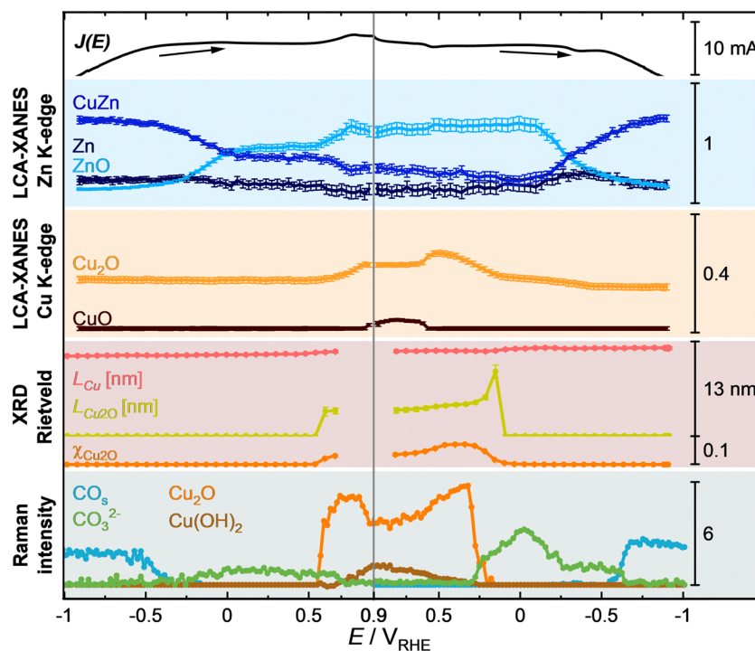
Fig. 5 Changes of the oxidation state and adsorbates during a CV extracted from operando measurements. Potential-dependent concentrations of CuZn, Zn, ZnO (Zn K-edge), \text{Cu}_2\text{O} , and CuO (Cu K-edge) from the LCA-XANES analysis of Zn K-edge and Cu K-edge XANES spectra (top), potential-dependent weight fraction of crystalline \text{Cu}_2\text{O} and volume-averaged crystallite sizes of Cu and \text{Cu}_2\text{O} obtained by Rietveld analysis of the HE-XRD patterns, and potential-dependent spectroscopic weight of adsorbates as \text{CO}_\text{s} and \text{CO}_3^{2-} and \text{Cu}_2\text{O} and \text{Cu}(\text{OH})_2 species obtained by fitting the normalized intensities (arb. units) of the bands from the SERS spectra. For XRD, the potential was already reversed at 0.7 V, while for XAS and SERS it was reversed at 0.9 V.
