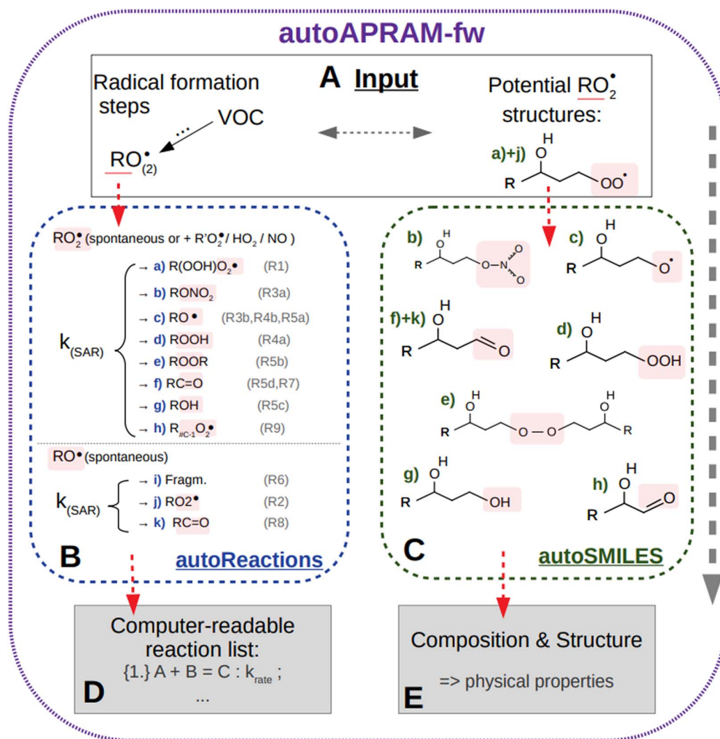
Fig. 1 Overview of the autoAPRAM-fw . Sector (A) represents the input to submodules autoReactions (B) and autoSMILES (C), respectively. Outputs comprise a Fortran readable chemistry module from autoReactions (D), and molecular information on the species formed in autoSMILES (E). Note that the submodules may be run individually.
