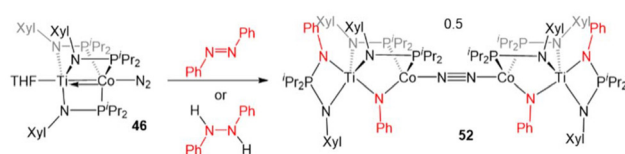
Scheme 13 N–N bond cleavage reaction of \text{Ti}^{\text{IV}}/\text{Co}^{\text{I}} compound 46 .
