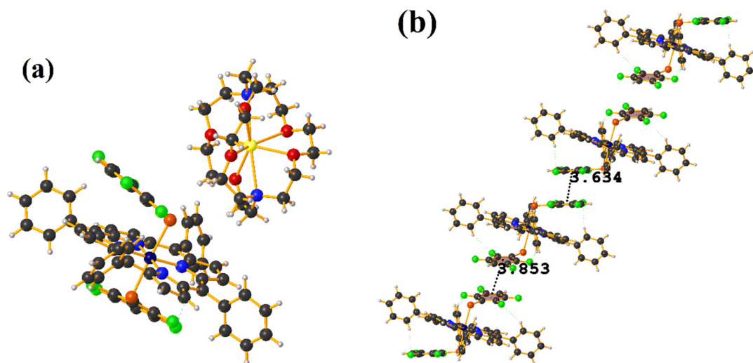
Fig. 14 (a) Molecular structure of COSJUP. For clarity, the numbering of the atoms is not shown. (b) Stacking interactions of COSJUP. For greater clarity, the molecule [NaC 22 ] is not shown.
