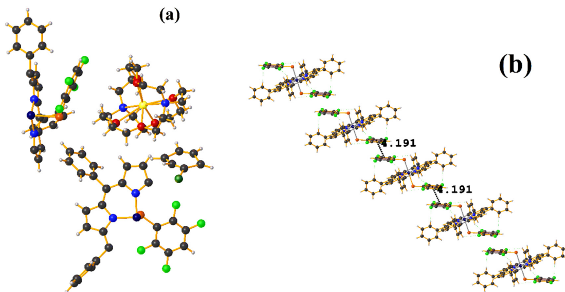
Fig. 13 (a) Molecular structure of COSJOJ. For clarity, the numbering of the atoms is not shown. (b) Stacking interactions of COSJOJ. For greater clarity, the molecules [NaC 22 ] and C 6 H 5 Cl are not shown.
