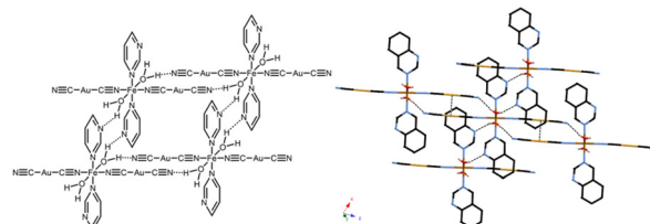
Fig. 3 Hydrogen bonding network of complex 2 .
