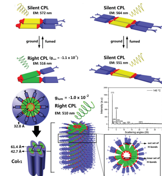
Fig. 14 Schematic illustration of thermo-mechanically induced CPL switching and LC assembly model for 4-10 and 4-11. Reproduced from ref. 105 with permission. Copyright (2020), The Royal Society of Chemistry.
