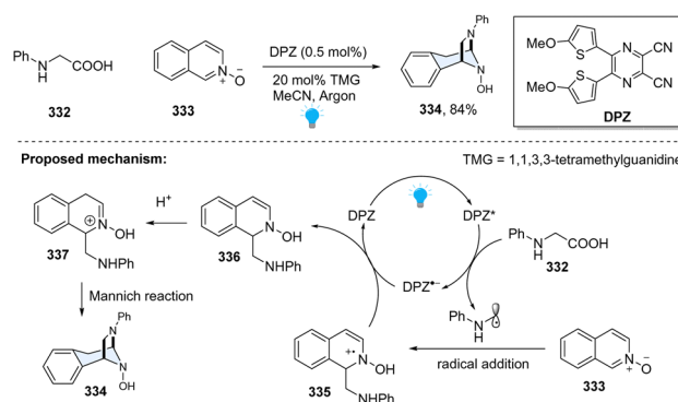
Scheme 34 Photoredox catalysed dearomative [3+2] cycloaddition of isoquinoline N -oxide.
