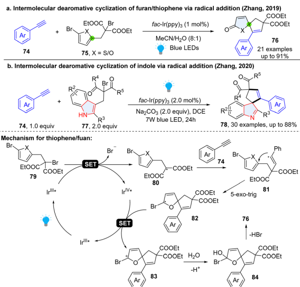
Scheme 12 Dearomative radical spirocyclization of electron rich thiophenes/furans/indoles.
