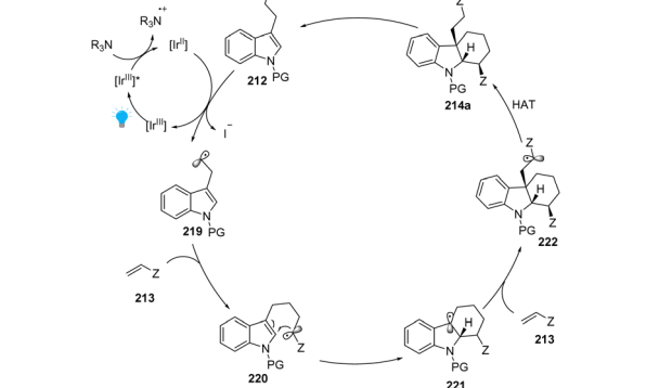
Scheme 24 Photoredox catalyzed cascade dearomative 2,3-difunctionalization of indoles using alkenes as a trapper.
