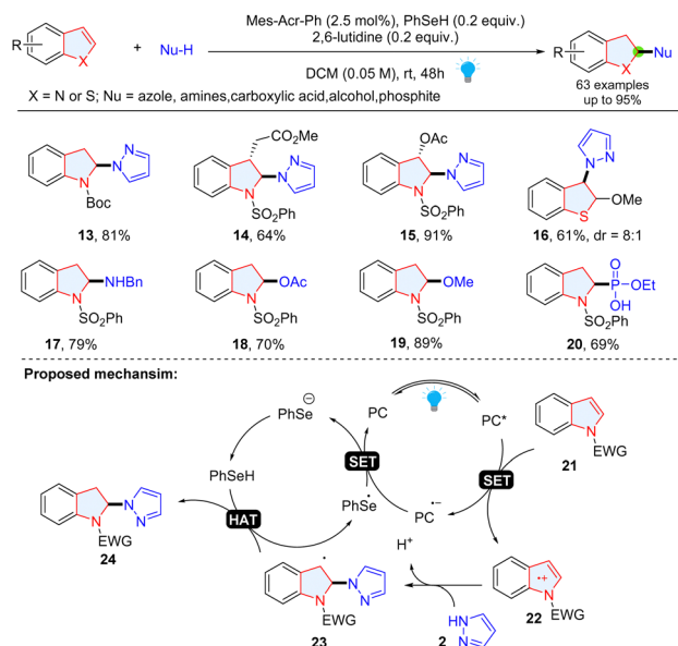
Scheme 5 Upmolung strategy enabled dearomative functionalization of indoles/thiophenes.
