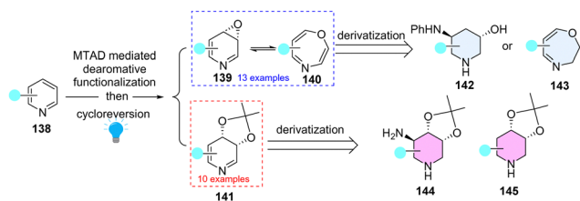
Scheme 17 Arenophile mediated dearomative multi-functionalization of pyridines.
