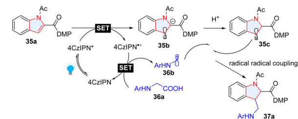
Scheme 8 Radical-radical coupling for dearomatization of electron deficient indoles.
