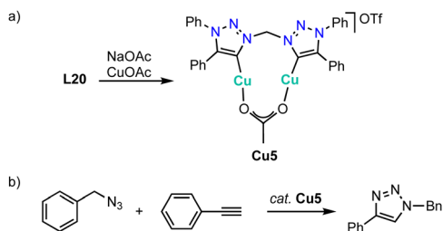
Scheme 39 (a) Synthesis of the bimetallic copper complex Cu5 with bridging bis(trz) and \text{OAc}^- ligands; (b) click reaction between phenyl acetylene and benzyl azide catalyzed by complex Cu5 .
