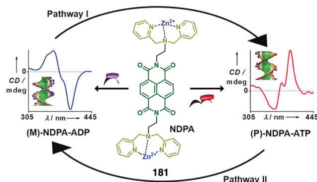
Fig. 89 Chemical structure of naphthalene diimide 181 , bearing as substituents zinc-complexes, that promotes P or M helical co-assemblies by interaction with ATP or ADP respectively. Reproduced from ref. 438 with permission from John Wiley and Sons, copyright 2017.
