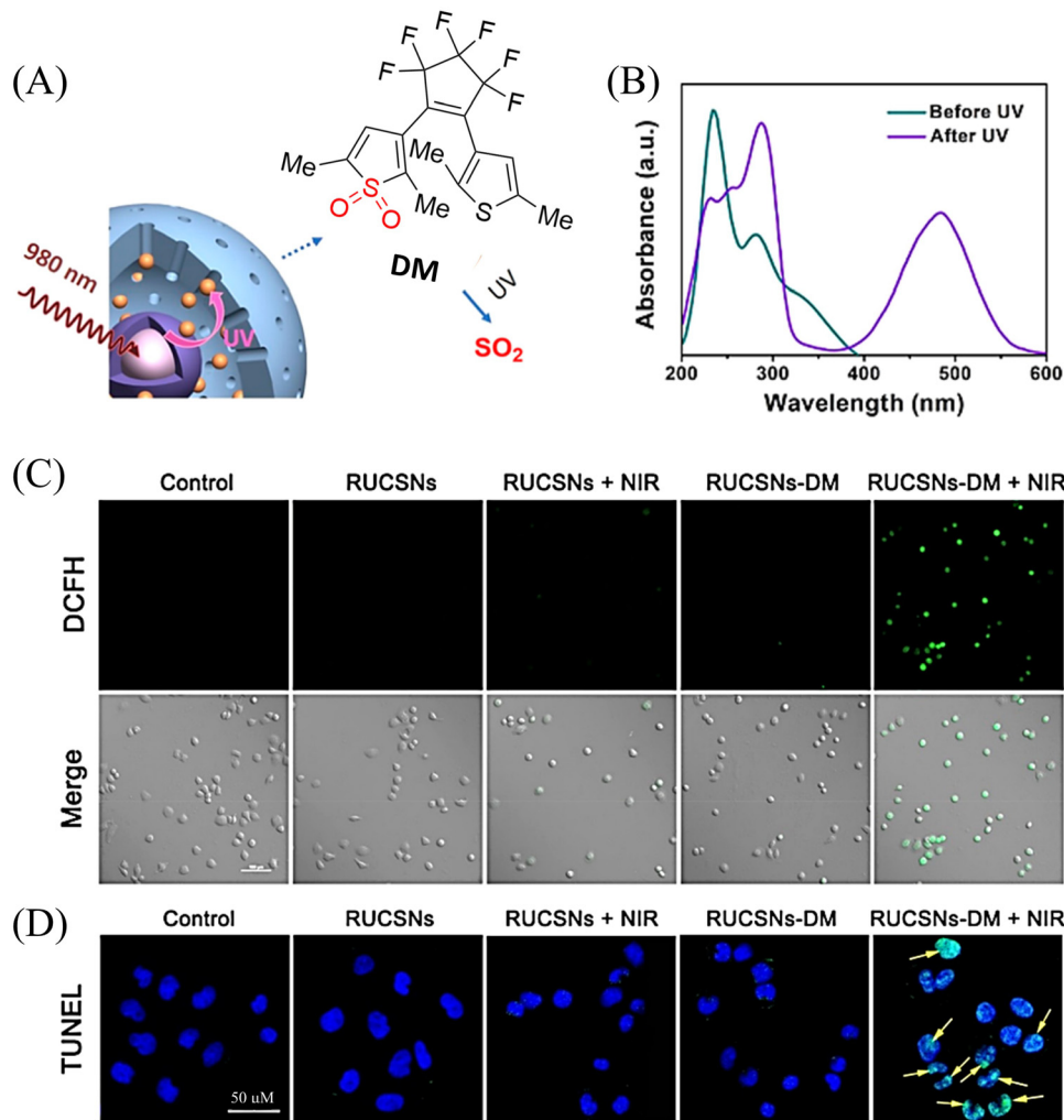
Fig. 73 (A) Schematic illustration of NIR light-triggered SO 2 generation from RUCSNs-DM. (B) UV-vis absorption spectra of DM before and after UV irradiation (365 nm). (C) Confocal imaging of intracellular ROS levels in HeLa cells after treatment with PBS (control), RUCSNs, RUCSNs + NIR (980 nm laser irradiation), RUCSNs-DM, RUCSNs-DM + NIR (980 nm laser irradiation) (D) Intracellular TUNEL staining in HeLa cells after treatment with different formulations (blue fluorescence: DAPI, green fluorescence: TUNEL). The yellow arrows indicated the overlap of blue fluorescence from DAPI and the green fluorescence from TUNEL, suggesting DNA fragmentation in the nucleus. Parts (A–D) are reproduced from ref. 208 with the permission of the American Chemical Society, copyright 2019.
