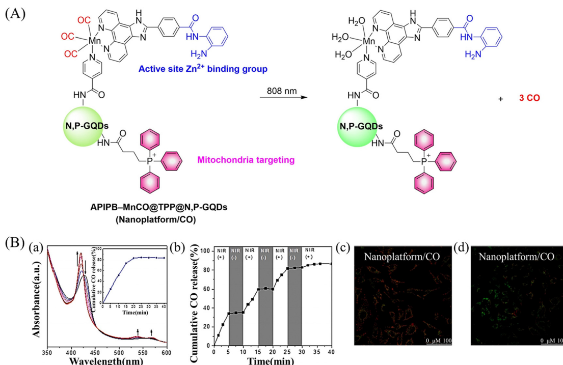
Fig. 31 (A) The structure of \text{APIPB-MnCO@TPP@N,P-GQDs} , the mechanism of CO release and its fluorescence changes. (B) (a) The absorbance change of hemoglobin in the presence of \text{Nanoplatform/CO} irradiated by 808 nm laser ( 800 \text{ mW cm}^{-2} ), with the inset showing the CO release profiles. (b) The NIR controllability of \text{Nanoplatform/CO} for CO release upon the on/off switching of an 808 nm laser. Fluorescence detection of mouse mitochondrial membrane potential, \text{Nanoplatform/CO} treated HeLa cells (c) under dark environment and (d) under 808 nm laser irradiation. Reproduced from ref. 109 with the permission of Elsevier Inc., copyright 2022.
