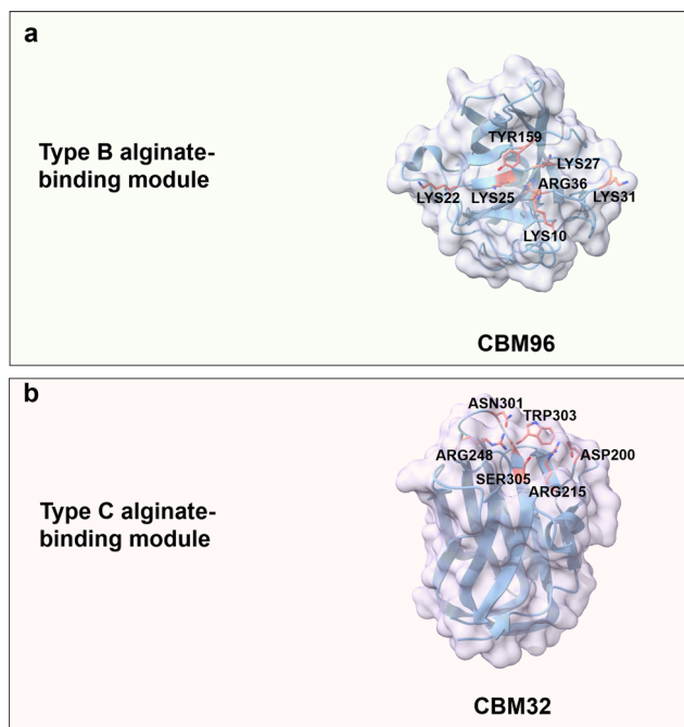
Fig. 9 Structures and key amino acids for alginate-binding modules. (a) Type B alginate-binding module that binds to alginate pentasaccharide. Representative CBM is CBM96 from Deftluviitalea phaphyphila alginate lyase (PDB: 7VBO), 154 which has a groove-shaped binding site. (b) Type C alginate-binding module that binds to alginate trisaccharide. Representative CBM is CBM32 AlyQ B from Persicobacter sp. CCB-QB2 alginate lyase (PDB: 7D2A), 14,155 which has a narrow binding pocket. Key residues for alginate binding interactions are highlighted in red. Protein models are visualized and coloured by ChimeraX 1.4. 46
