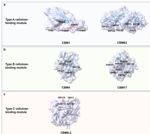
Fig. 4 Structures and key amino acids in cellulose binding in the three main cellulose-binding modules (type A–C). (a) Type A cellulose-binding modules that bind to cellohexaose. Representative CBMs are CBM1 from Trichoderma reesei cellobiohydrolase I (PDB: 1CBH) 51,54 and CBM63 from Bacillus subtilis expasin, 50 which have a planar-shaped binding site. (b) Type B cellulose-binding modules that bind to cellobextrin and cello-tetraose respectively. Representative CBMs are CBM4 from Clostridium thermocellum CbhA (PDB: 3K4Z) 55 and CBM17 from Clostridium cellulovorans Cel5A (PDB: 1J84), 56 which have a cleft- or groove-shaped binding site. (c) Type C cellulose-binding module that binds to cellobiose. Representative CBM is CBM9-2 from Thermotoga maritima xylanase 10 A (PDB: 1I82), 57 with a narrow binding pocket. Key residues for cellulose binding interactions are highlighted in red. CBM structures without specified PDB IDs are predicted with AlphaFold2. 58 Protein models are visualized and coloured by ChimeraX 1.4. 46
