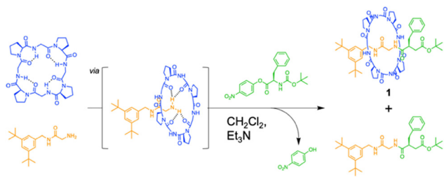
Fig. 16 Synthesis of an all peptide-based [2]rotaxane by the cyclic peptide-accelerated N -acylation of primary amines. Reproduced with permission from ref. 101 Copyright 2024, American Chemical Society.
