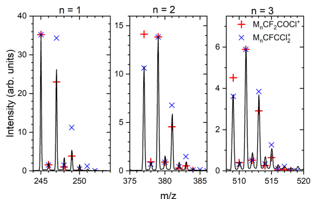
Fig. 4 Details of the mass spectrum of (\text{CF}_3\text{COCl})_n clusters for the ambiguous series \text{M}_n\cdot\text{R}^+ where \text{R} = \text{CF}_2\text{COCl} or \text{CFCCl}_2 (orange triangles in Fig. 3). Symbols indicate the calculated abundances of the isotopes normalized to the maximum peak within each group.
