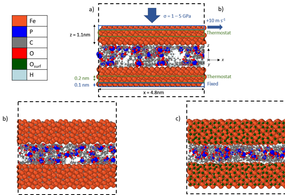
Fig. 2 Side-view snapshots showing the model systems with TCP molecules confined between (a) \alpha -Fe(110), (b) \text{Fe}_3\text{C}(010) , and (c) \text{Fe}_3\text{O}_4(001)\text{-SCV} surfaces. Systems shown after minimisation and equilibration, but before heating, compression, and shear. Black dashed line shows the simulation box. Rendered using OVITO. 42
