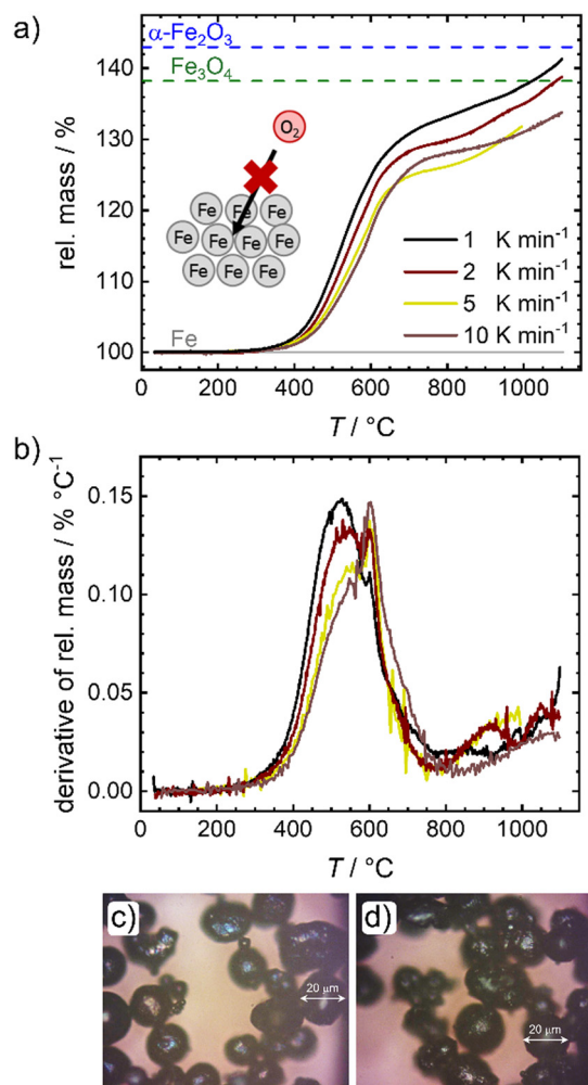
Fig. 2 (a) Temperature programmed oxidation and (b) related derivatives for different heating rates. For reasons of comparison the mass gain assigned to a full oxidation to Fe 3 O 4 and α-Fe 2 O 3 is added. (c) and (d) Photographs of the samples obtained from oxidation under constant heating in a tube oven with 1 K min −1 up to 300 °C (c) and 600 °C (d).
