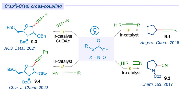
Fig. 9 Decarboxylation of aliphatic acids for C(sp^3)-C(sp) cross-coupling.
