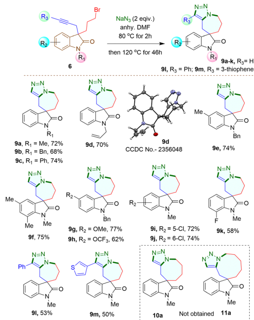
Scheme 5 Synthesis of triazolo azepine-containing spirooxindoles from 3,3-disubstituted oxindoles. Reaction conditions: 6 (0.15 mmol), \text{NaN}_3 (0.30 mmol) in anhydrous DMF (1 mL) at 80 °C for the first 2 hours, then another 46 hours at 120 °C. Isolated yields.
