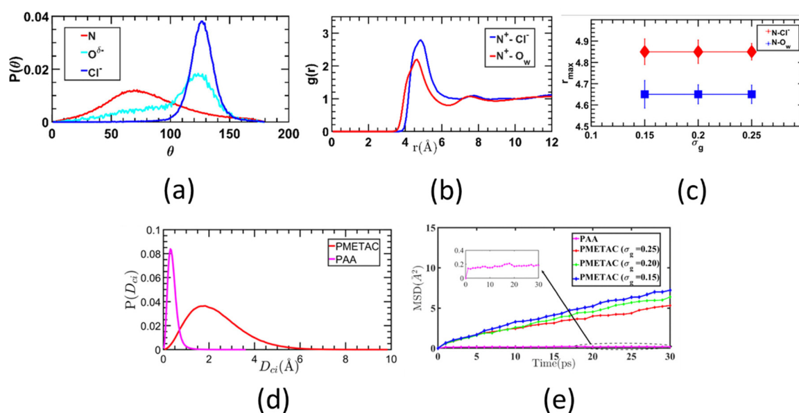
Fig. 23 (a) Dipole orientation of water molecules around the \{N(\text{CH}_3)_3\}^+ functional group of the PMETA chain, \text{C}=\text{O} (ester group) of the PMETA chain, and the \text{Cl}^- counterions that screen the PMETA brush charges. (b) Comparison of the radial distribution function of \text{N}^+-\text{Cl}^- and \text{N}^+-\text{O}_w [here \text{N}^+ is the nitrogen atom of the \{N(\text{CH}_3)_3\}^+ group and \text{O}_w is the oxygen atom of the water molecule]. (c) Variation of the peak locations of the \text{N}^+-\text{Cl}^- and \text{N}^+-\text{O}_w with grafting density. (d) Probability distribution function of the distance travelled by the \text{Na}^+ counterion (in the PAA brush environment) with \text{Cl}^- counterion (in the PMETAC brush environment). (e) MSD-vs.-time variation for the \text{Na}^+ counterion (in the PAA brush environment) with \text{Cl}^- counterion (in the PMETAC brush environment; for this case, results have been provided for different PMETAC grafting densities). All the parts of the figure have been reprinted with permission from Ishraaq, R.; Akash, T. S.; Bera, A. K.; Das, S., Hydrophilic and Apolar Hydration in Densely Grafted Cationic Brushes and Counterions with Large Mobilities, The Journal of Physical Chemistry B , 2024, 128 (1), 381–392. Copyright (2023) American Chemical Society.
