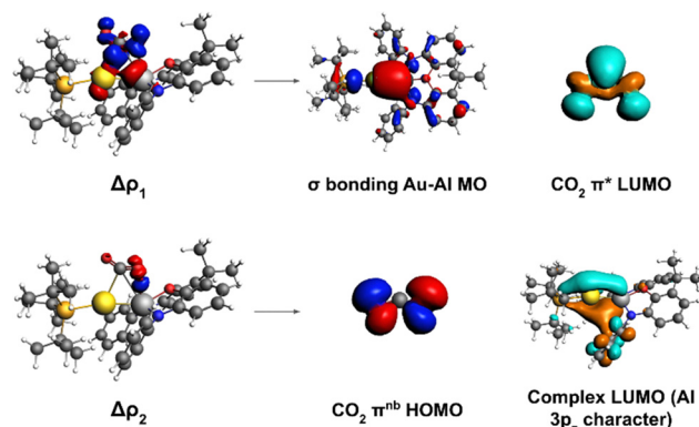
Fig. 2 Left: Isodensity surfaces associated with the Δρ 1 and Δρ 2 NOCV deformation densities for the transition state structure TSI. The charge flux is red-to-blue. The isodensity value is 5 m e a 0 −3 for both surfaces. Right: Most significant contributions from the [ t Bu 3 PAuAl(NON)] and CO 2 fragments molecular orbitals (MOs) to the interactions described by the NOCV deformation densities. Isodensity values for all MO isosurfaces is 30 m e a 0 −3 . All isosurfaces are taken and adapted with permission from ref. 30 Copyright 2021, American Chemical Society.
