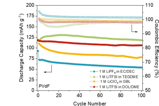
Fig. 8 DAAQ-TFP-COF electrode performance with PVdF as a binder at 150 mA g -1 (1C) in four different electrolytes: 1 M LiTFSI in DOL/DME (1:1, vol%) (red), 1 M LiTFSI in TEGDME (green), 1 M LiPF 6 in EC/DEC (1:1, vol%) (blue), and 1 M LiClO 4 in GBL (yellow). Adapted with permission from ref. 85.
