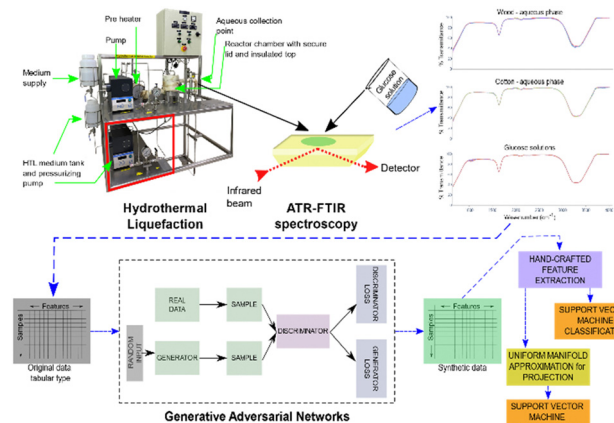
Fig. 1 The overall workflow of the HTL process with the application of GAN for synthetic data generation. The ATR-FTIR generated spectrum datasets were pre-processed, scaled, and passed through GAN. The original datasets were merged with the synthetic data forming a hybrid dataset. Hand-crafted feature extraction based on statistical features was employed to extract extra information from the spectrums. UMAP was then used to reduce the data to the most significant features. Ultimately, we applied support vector machines (SVC) to build a classification model. The feature importance was explained using SHAP.
