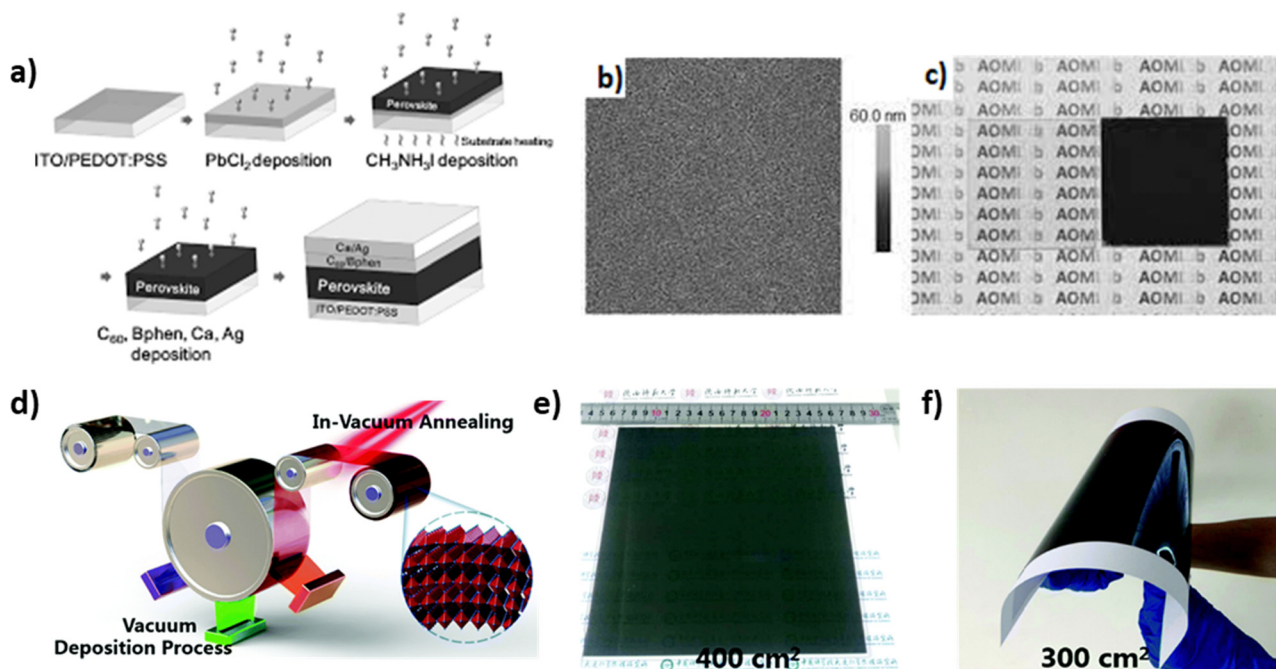
Fig. 5 (a) Schematic illustration of perovskite solar cells fabricated by sequential layer-by-layer vacuum deposition. (b) AFM image (30 \mu\text{m}^2 ) of the vacuum-deposited \text{PbCl}_2 thin film. (c) Photographs of the vacuum deposited \text{PbCl}_2 (left) and perovskite (right) thin films. Adapted with permission from ref. 102. (d) Schematic illustration of multisource vacuum deposition with an in-vacuum annealing process for large-area perovskite films. Photographs of FA-based perovskite films deposited on (e) glass and (f) PET substrates. Adapted with permission from ref. 104.
