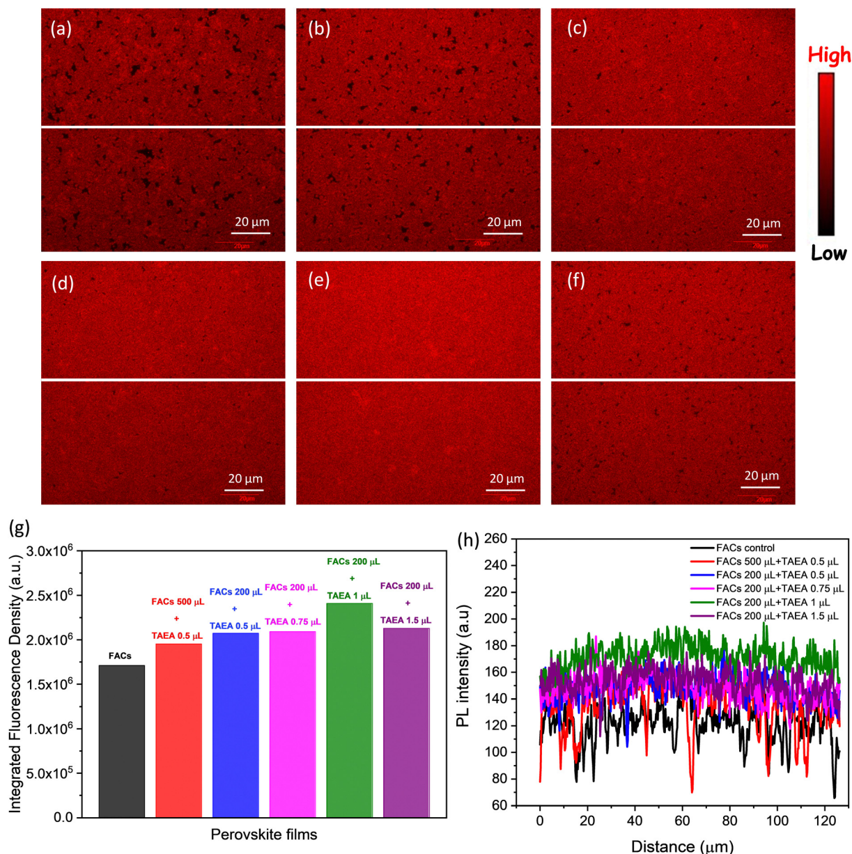
Fig. 5 SLCM PL intensity maps of (a) FACs film, FACs film containing (b) 0.5 \mu\text{L} of TAEA in 500 \mu\text{L} of FACs precursor, (c) 0.5 \mu\text{L} of TAEA in 200 \mu\text{L} of FACs precursor, (d) 0.75 \mu\text{L} of TAEA in 200 \mu\text{L} of FACs precursor, (e) 1 \mu\text{L} of TAEA in 200 \mu\text{L} of FACs precursor, and (f) 1.5 \mu\text{L} of TAEA in 200 \mu\text{L} of FACs precursor. (g) Integrated fluorescence density in the films calculated in the 128 \mu\text{m} \times 128 \mu\text{m} area of the sample. (h) PL line profile plotted along the breadth of the samples as denoted by the white horizontal lines in (a)–(f).
