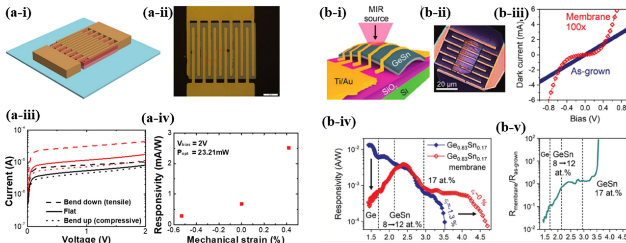
Fig. 5 (a) Device structure and characteristics of flexible GeSn metal semiconductor metal (MSM) NM PD. 19 (i) & (iii) Schematic and an optical image of the device structure, (iii) dark current and photocurrent under flat and bending conditions, and (iv) responsivity at 2000 nm as a function of mechanical strains. Reproduced with permission from ref. 19. Copyright 2020, Royal Society of Chemistry. (b) Structure and characteristics of GeSn NM PD on SiO 2 /Si: (i) & (ii) Schematic and an optical image of a fabricated device, (iii) dark current versus bias voltage, (iv) responsivity versus wavelength of as-grown and membrane devices, and (v) spectral responsivity ratio of the membrane and the as-grown GeSn device. 63 Reproduced with permission from ref. 63. Copyright Copyright 2020, Wiley-VCH.
