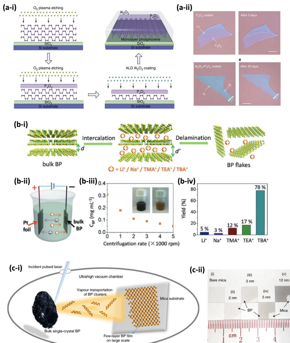
Fig. 8 (a) Mechanically exfoliated black phosphorus (BP) on a SiO 2 /Si substrate treated with O 2 plasma etching: (a-i) schematic illustration of the preparation process, and (a-ii) OM images of single-layer BP covered by P 2 O 5 or P 2 O 5 /Al 2 O 3 capping layer before and after several days. 109 Reproduced with permission from ref. 109. Copyright 2016, Springer Nature. (b): Electrochemically exfoliated BP: (b-i) Schematic delamination procedure, (b-ii) Experimental setup, (b-iii) Concentration of BP as a function of centrifugation rate, and (b-iv) Delamination yield as a function of intercalating cations. 125 Reproduced with permission from ref. 125. Copyright 2016, John Wiley-VCH.
