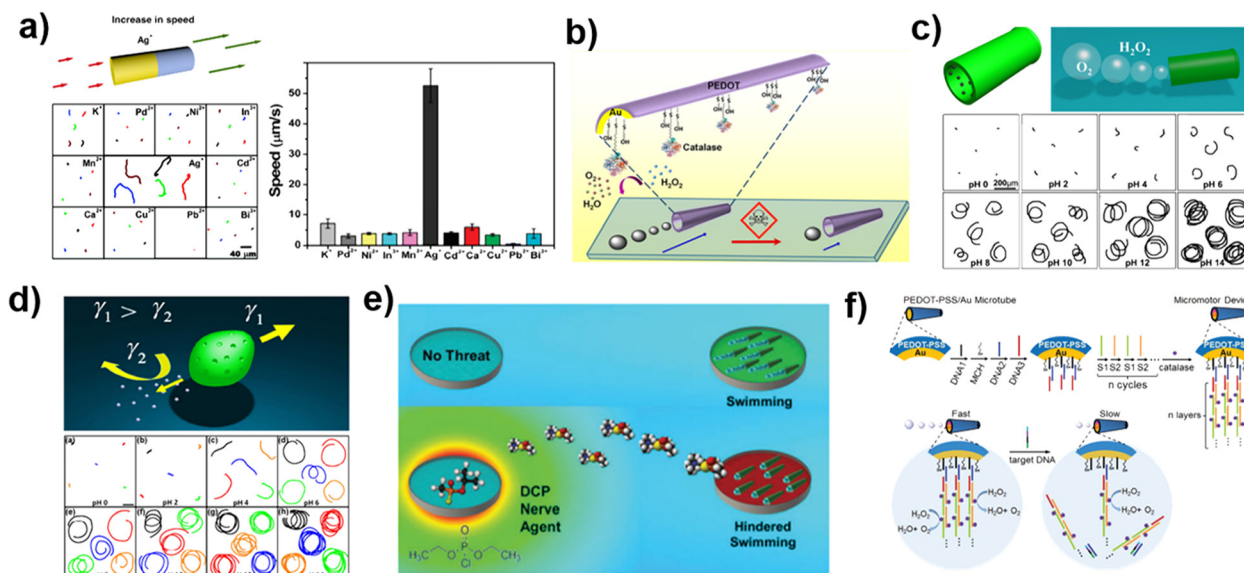
Fig. 2 Sensing based on the motion behavior analysis of MNMs. (a) Metal ion response using gold-platinum nanomotors based on motion changes. Reprinted from ref. 69 with permission of the American Chemical Society, copyright 2009. (b) Scheme illustrating the pollutant inhibiting the activity of catalase powered micromotors. Reprinted from ref. 25 with permission of the American Chemical Society, copyright 2013. (c) pH responsive bullet-shell motor based on motion changes. Reprinted from ref. 71 with permission of the American Chemical Society, copyright 2016. (d) Spindle-shaped motor for pH sensing based on motion change. Reprinted from ref. 72 with permission of Springer, copyright 2016. (e) The detection of diethylphosphorochloride was achieved by peroxidase powered motors. Reprinted from ref. 74 with permission of the Royal Society of Chemistry, copyright 2016. (f) Micromotors for DNA detection based on motion changes. Reprinted from ref. 77 with permission of the Royal Society of Chemistry, copyright 2017.
