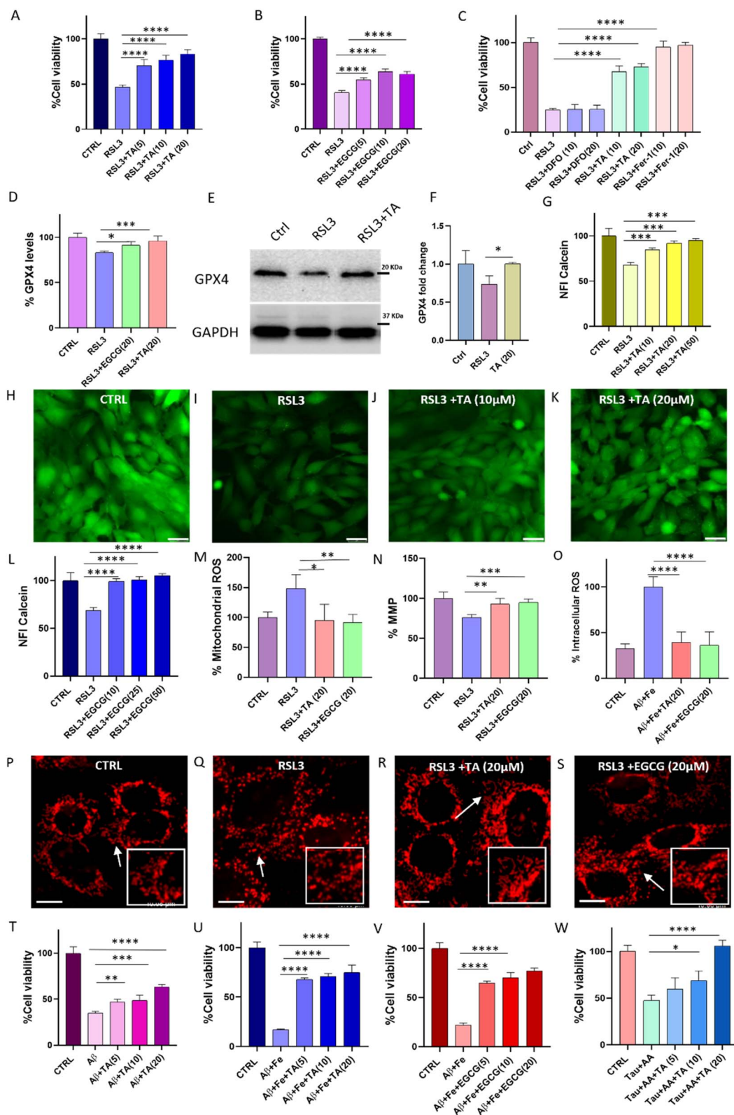
Fig. 5 Studies in cells show the ability of TA and EGCG to rescue neuronal cells from ferroptosis and A \beta 42 -induced toxicity. The numbers in the parentheses represent the concentration of the compounds in \mu M. Neuronal cell rescue from RSL3 (500 nM) induced ferroptosis by (A) TA and (B) EGCG, (C) comparative study with ferrostatin and DFO, (D) immunofluorescence (IF) study to monitor relative GPX4 levels in cells treated with RSL3 (1 \mu M) alone and in the presence of TA (20 \mu M) and EGCG (20 \mu M), and (E) western blot and its quantification to monitor GPX4 levels (F) ( n > 3 ). (G) Monitoring LIP using calcein and visualization of LIP in (H) control, (I) RSL3 (2 \mu M), (J) RSL3 + TA (10 \mu M) and (K) RSL3 + TA (20 \mu M) treated cells (scale bar: 30 \mu m), (L) monitoring LIP in the presence of EGCG using Calcein-AM, (M) intracellular mitochondrial ROS levels monitored using MitoSOX in cells treated with RSL3 (1 \mu M) alone and in the presence of TA (20 \mu M) and EGCG (20 \mu M), (N) MMP monitored using Mitotracker green
