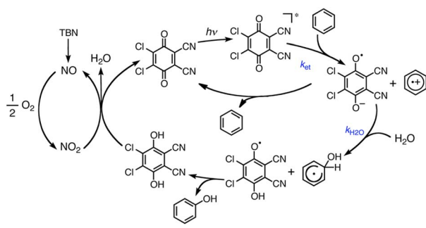
Scheme 7 A mechanism for photohydroxylation of benzene by dioxygen with DDQ used as a photoredox catalyst in the presence of TBN and H 2 O in MeCN under photoirradiation. Reprinted from ref. 44 with permission from American Chemical Society (Copyright 2013).
