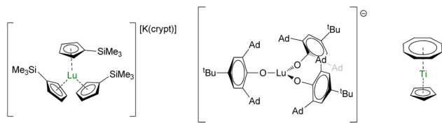
Fig. 10 Molecular structures of [Lu(Cp*)(crypt)] + , 217 [Lu(OAr*) 3 ] - , 218 and (Cp)Ti(Cot). 213
