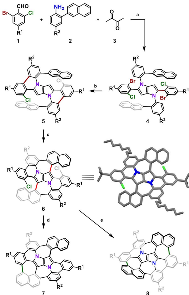
Scheme 1 Synthetic route to molecular saddle 8 . Reagents and conditions: (a) Fe(ClO 4 ) 3 ·xH 2 O (6 mol%), AcOH/toluene, 50 °C, 16 h, 49%; (b) Pd(OAc) 2 (20 mol%), Cs 2 CO 3 (2.4 equiv.), PPh 3 (48 mol%), toluene, 120 °C, 4 h, 91%; (c) Fe(OTf) 3 (6.0 equiv.), DCE/MeNO 2 , 80 °C, 6 h, 24%; (d) Pd(OAc) 2 (2.0 equiv.), HPt-Bu 2 MeBF 4 (6.0 equiv.), DBU/DMA, 180 °C, 24 h, 52%; (e) t -BuOK (10.0 equiv.), DMSO, blue LEDs, rt, 20 h, 75%. DMA – dimethylacetamide, DCE – 1,2-dichloroethane; inset: X-ray crystal structure of 6 . R 1 = t -Bu, R 2 = n -C 8 H 17 .
