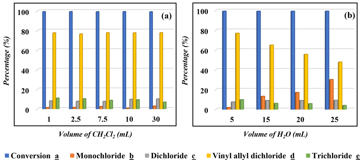
Fig. 3 Effect of dilution of (a) CH 2 Cl 2 and (b) H 2 O on the selective catalytic chlorination of carvone a .
