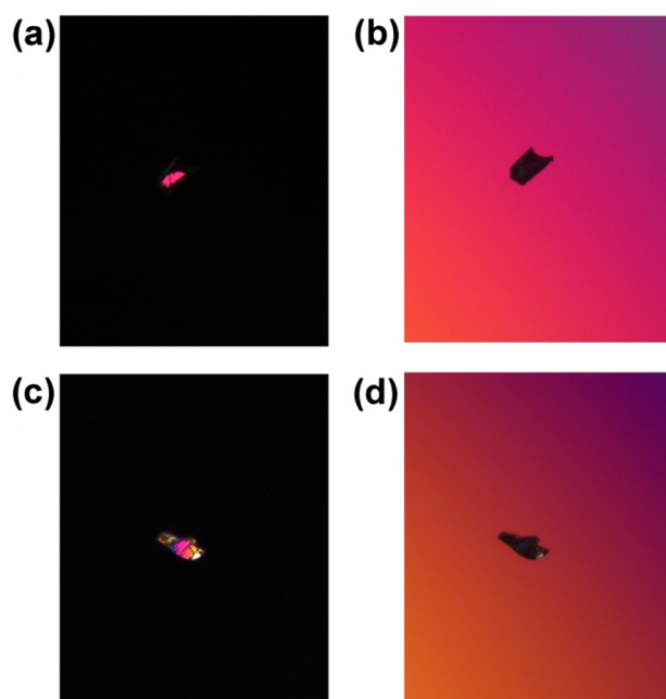
Fig. 3 (a and b) \text{Ba}_3\text{MnGe}_3\text{O}_{28}\text{S}_8 and (c and d) \text{Ba}_3\text{CdGe}_3\text{O}_{28}\text{S}_8 crystals for birefringence determination and the interference colors observed before and after complete extinction.
