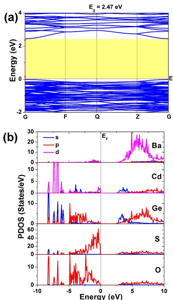
Fig. 4 Theoretical calculated results of \text{Ba}_3\text{CdGe}_3\text{O}_{28}\text{S}_8 : (a) electronic band structure; (b) PDOS curve.
